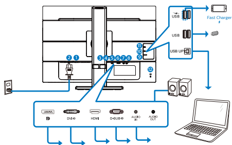
USB hub
