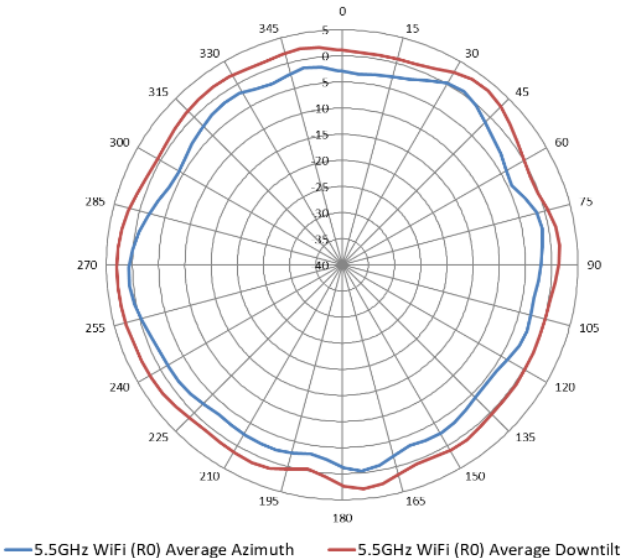
5.5 GHz Wi-Fi antenna patterns (horizontal)
