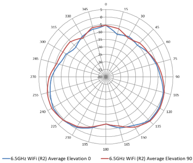
6.5GHz Wi-Fi antennas patterns (vertical)
