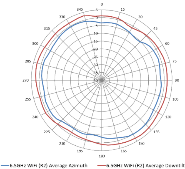
6.5 GHz Wi-Fi antenna patterns (horizontal)
