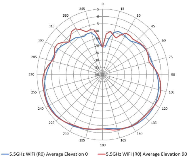
5.5GHz Wi-Fi antenna patterns (vertical)
