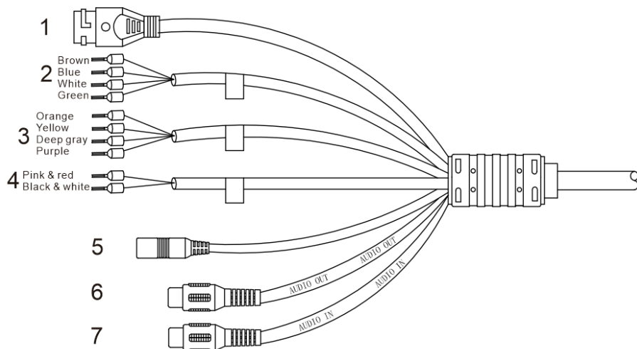
Figure 1-5 Multi-connector Combination Cables
