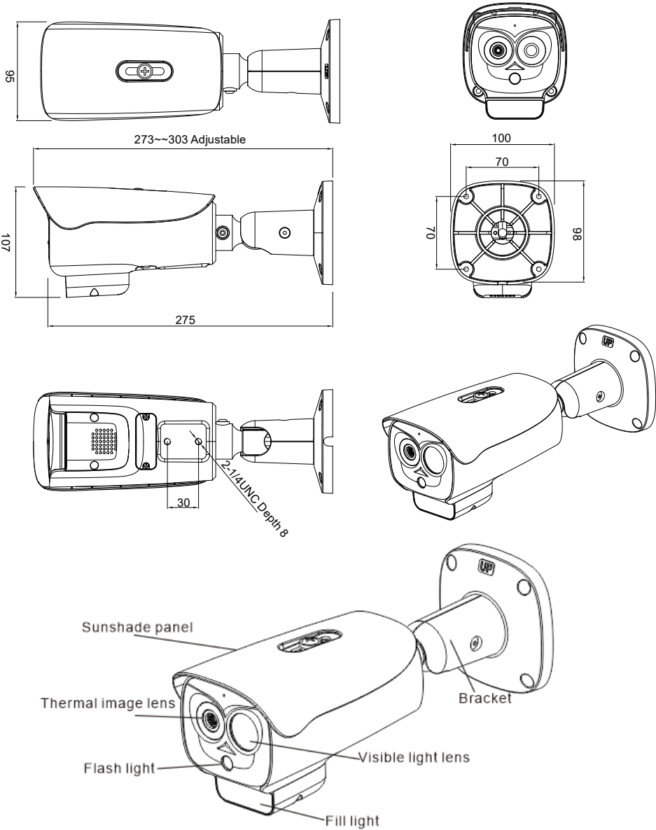
Figure 1-1 Dimensions (unit: mm)
